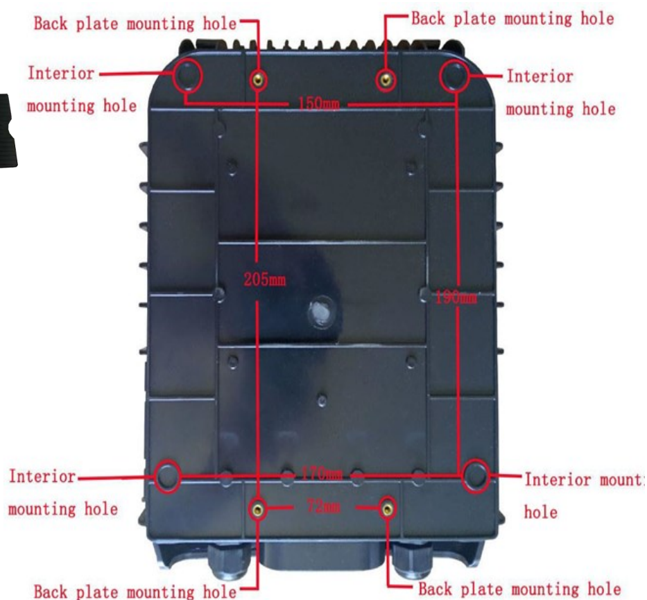
Product mounting hole
