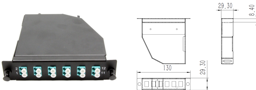
1xMPO/MTP-LC DX 12F
