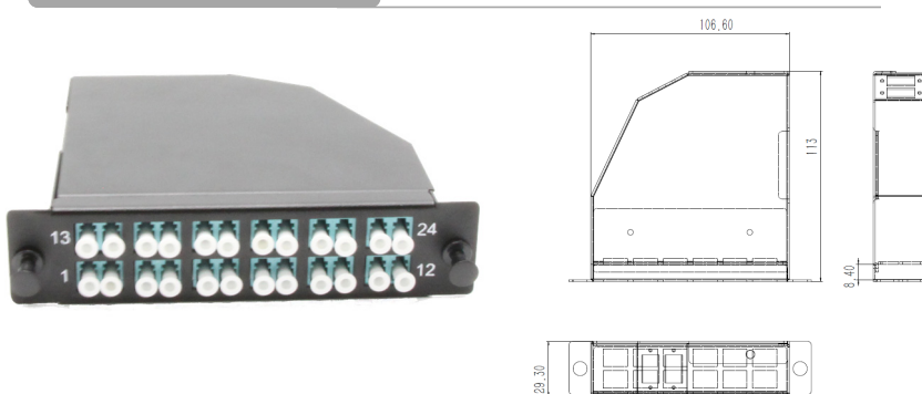
1xMPO/MTP-LC DX 24F
