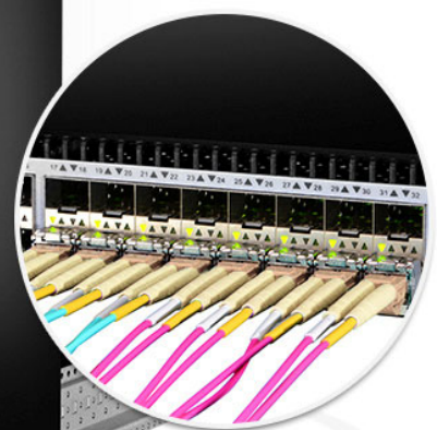
4× LC connectors for 10G SFP+
