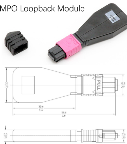
12 Fibers
