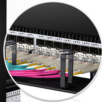
12× LC connectors for 10G SFP+
